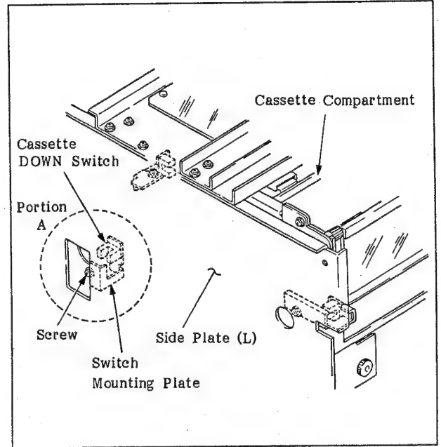
Fig. 6-18 Cassette DOWN Switch
